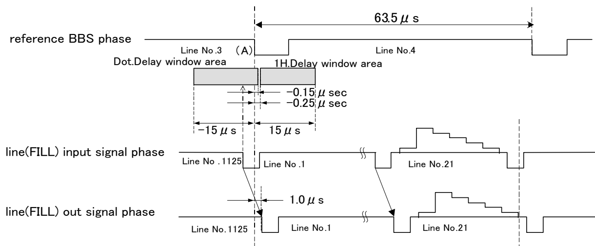
1080 i window area
