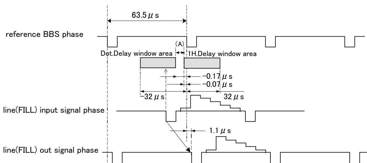
525i window area
