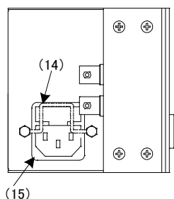
図3.5 MTX-70P-88側面図
