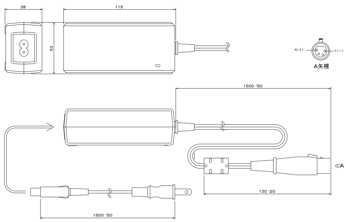
(2) VAC-12V04A
